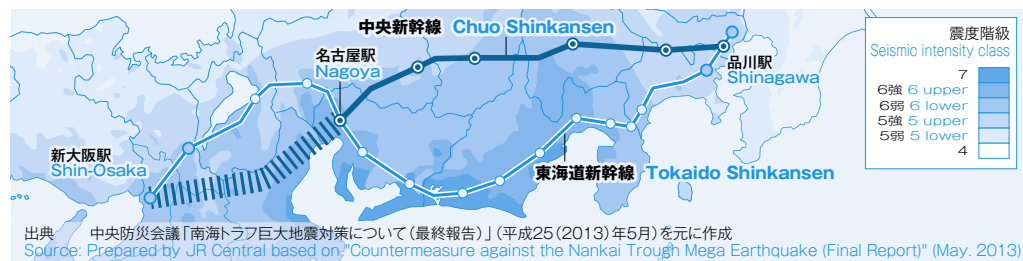
南海トラフ巨大地震の想定震度の最大値の分布図 Distribution map of the estimated biggest seismic intensity of the Nankai Trough Mega Earthquake
